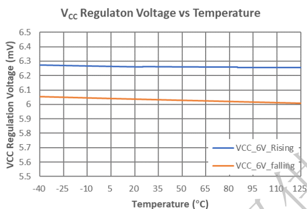
Figure 7. V_{CC} Regulation Voltage vs Temperature ( V_D=14V , HVIN=0V )
