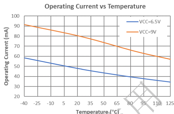
Figure 6. Operating Current vs Temperature ( C_{LOAD}=2.2nF , FSW=100kHz )
