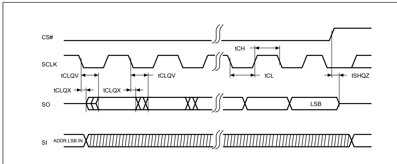
Figure 9. Output Timing
