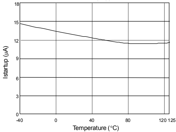
Fig. 9 Startup Current (I start ) vs. Temperature
