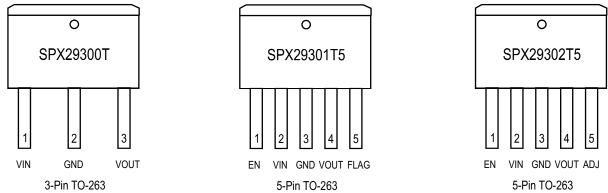
Figure 3: SPX29300, SPX29301, SPX29302 Pin Assignments
