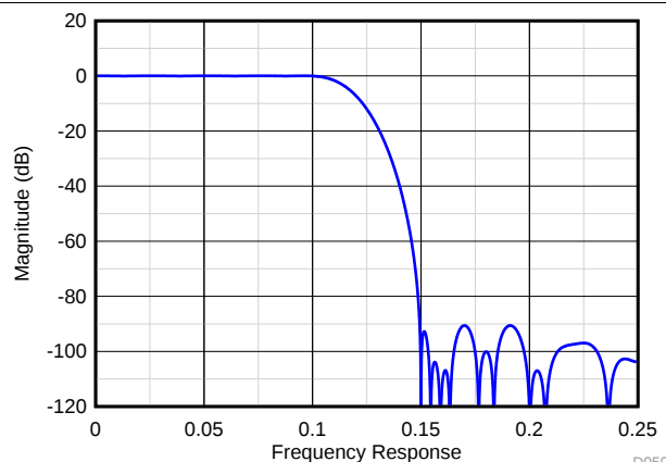
Figure 60. Frequency Response for Decimate-by-2 Low-Pass Filter (in Mode 4 and Mode 7)
