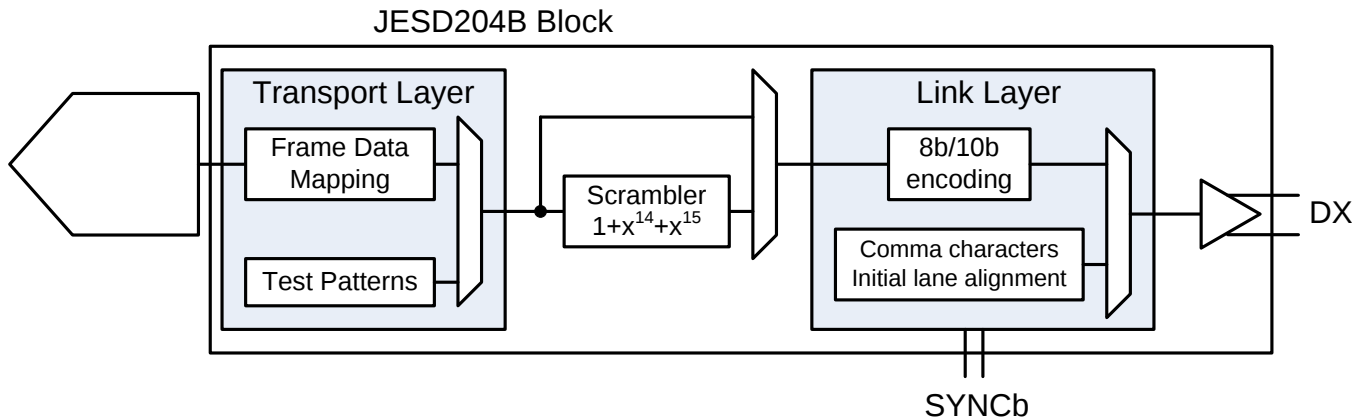
Figure 81. JESD Interface Block Diagram
