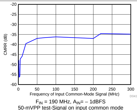
Figure 42. Common-Mode Rejection Ratio
