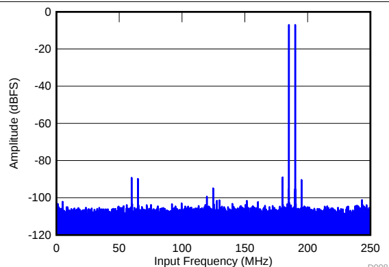
F_{\text{IN1}} = 185\text{ MHz} , F_{\text{IN2}} = 190\text{ MHz} , IMD = 89 dBFS Each tone at -7\text{ dBFS}
