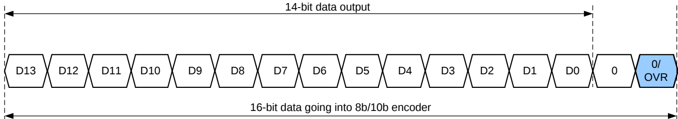
Figure 71. Timing Diagram for FOVR
