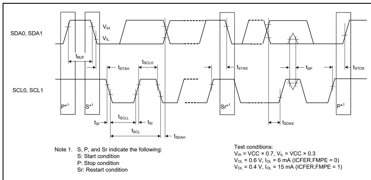
Figure 2.53 I 2 C bus interface input/output timing
