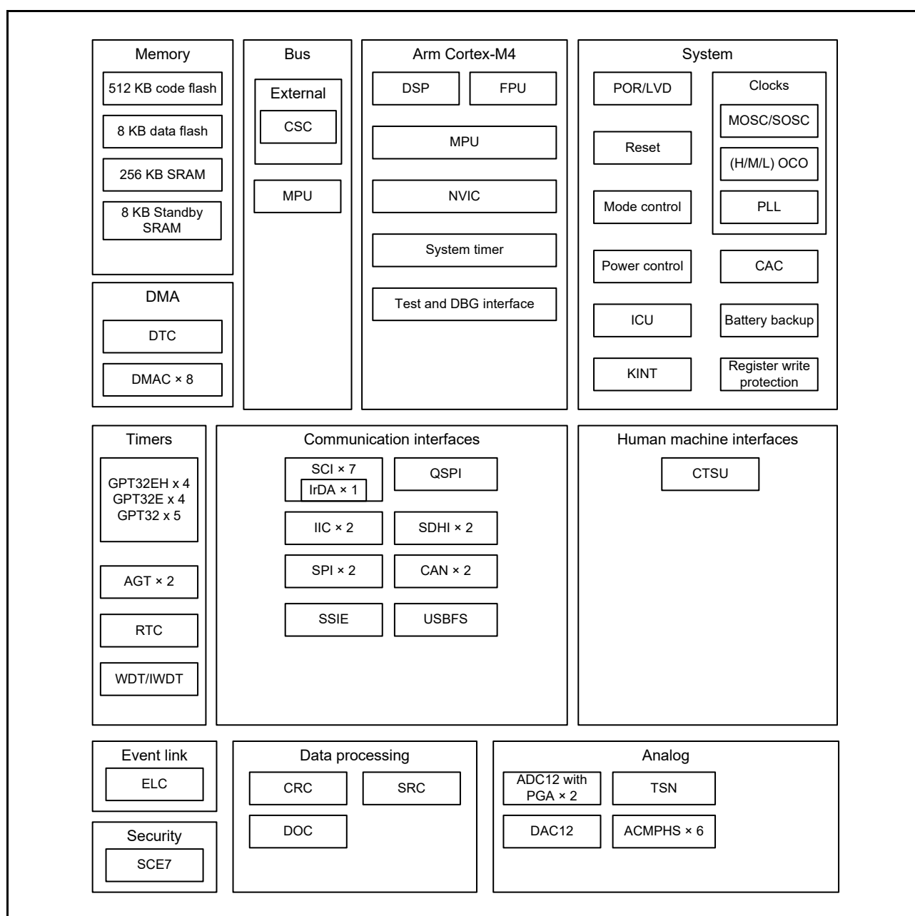
Figure 1.1 Block diagram
