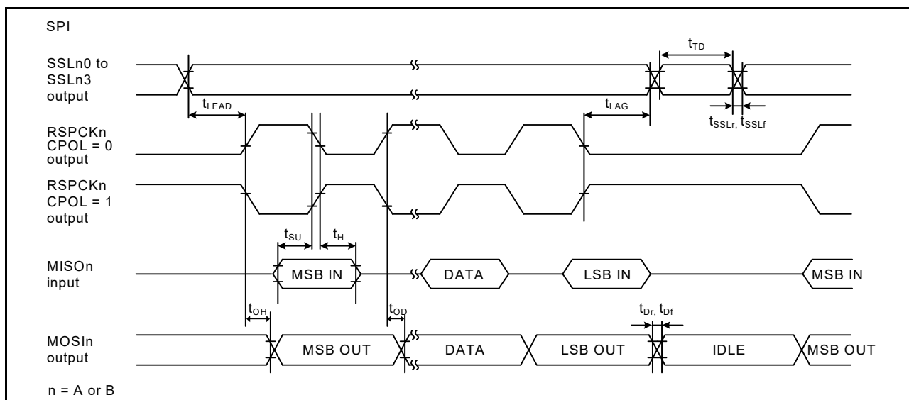
Figure 2.47 SPI timing for master when CPHA = 1
