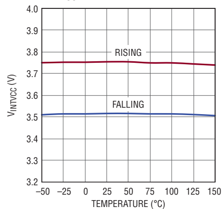
INTV CC UVLO Threshold
