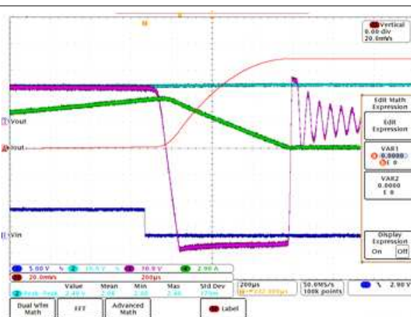
Figure 27. Inductive Load Switching-Off Expanded Waveform
