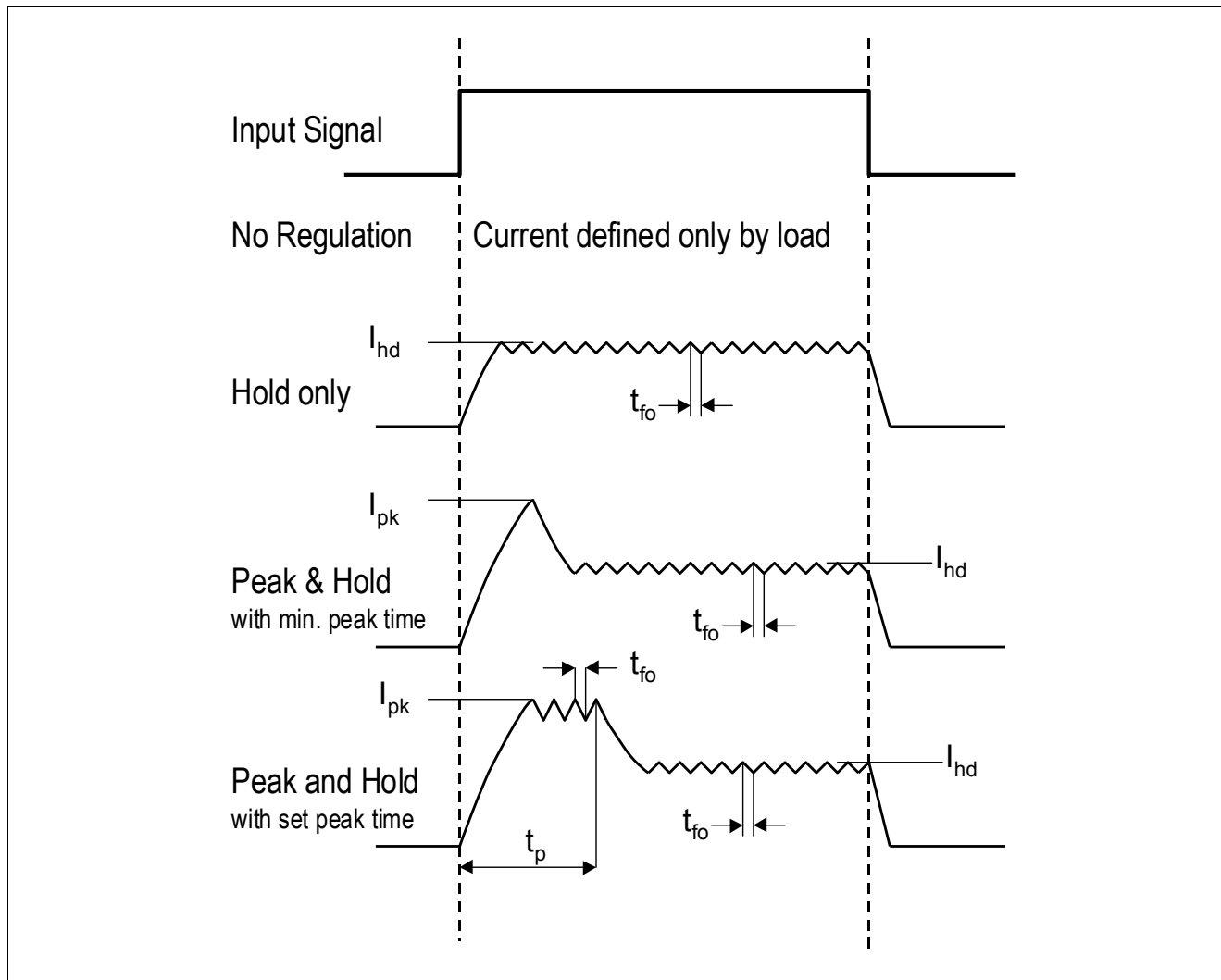
Figure 6 Current Forms of the Different Current Control Modes of Channel 1-3
