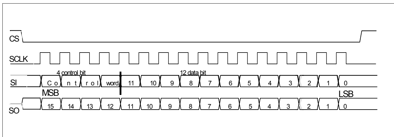
Figure 16 Serial Interface
