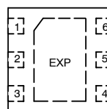
WDFN6 2x2 mm (Top View)
