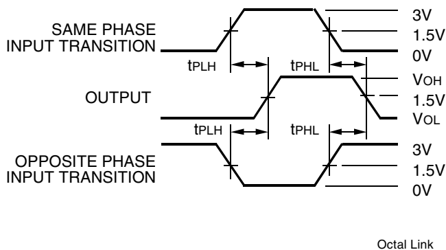
Propagation Delay
