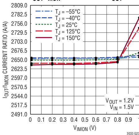
I_{OUT}/I_{MON} Current Ratio, I_{OUT} = 3A
