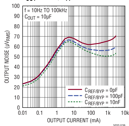
RMS Output Noise V_{\text{OUT}} = 0.2\text{V} , C_{\text{FF}} = 0
