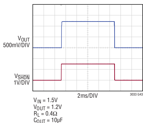
SHDN Transient Response C_{\text{REF/BYP}} = 0
