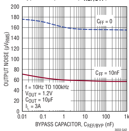
RMS Output Noise vs Bypass Capacitor ( C_{\text{REF/BYP}} )
