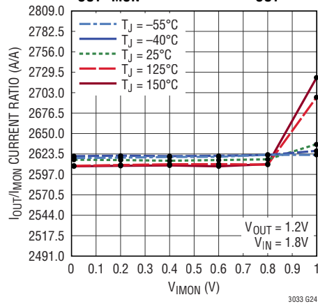
I_{OUT}/I_{MON} Current Ratio, I_{OUT} = 3A
