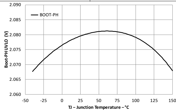
Figure 15. BOOT-PH UVLO vs Junction Temperature
