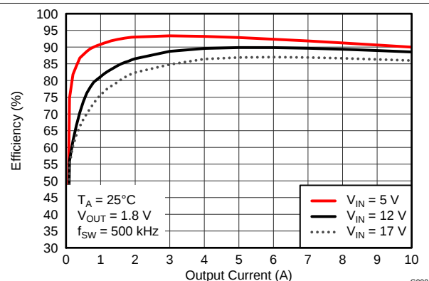
Figure 41. Efficiency
