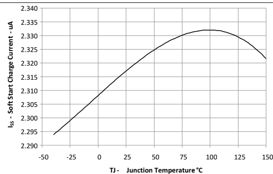
Figure 10. Soft-Start Charge Current vs Junction Temperature
