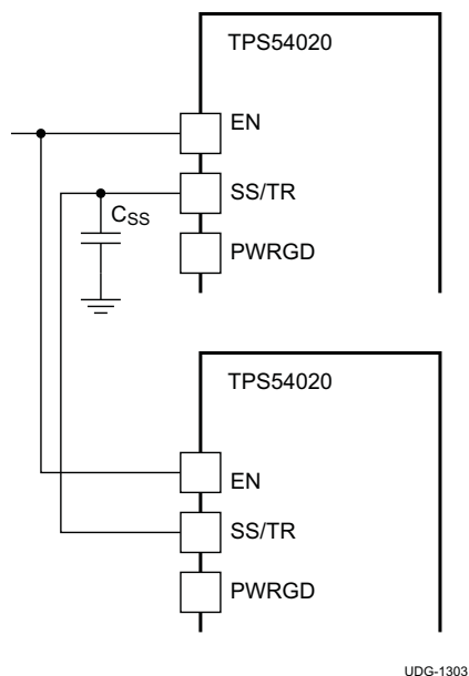
Figure 20. Ratiometric Start Up Sequence
