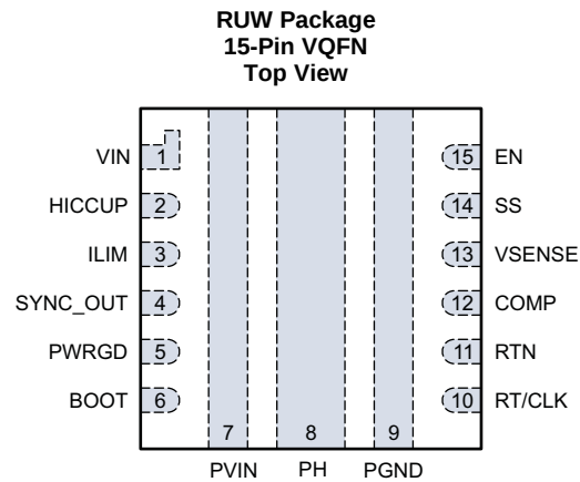
Pin Functions
