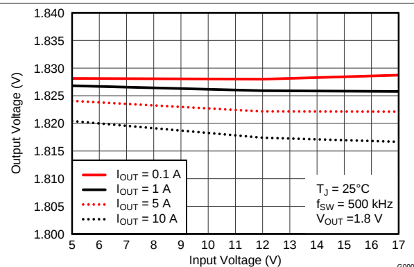
Figure 39. Line Regulation
