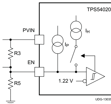
Figure 17. Adjustable PVIN Undervoltage Lockout, PVIN \geq 4.5\text{ V}
