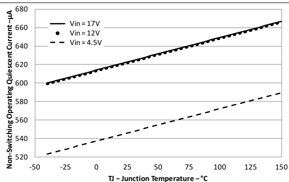
Figure 9. Nonswitching Operating Current vs Junction Temperature
