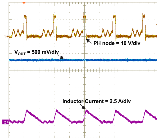
Figure 23. TPS54020 in Discontinuous Conduction Mode
