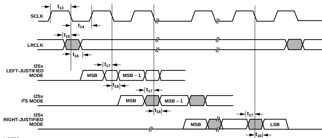
Figure 4. I²S Timing
