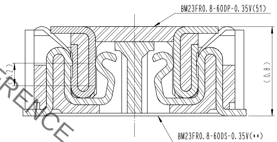
ENGAGEMENT FIGURE (50:1)
