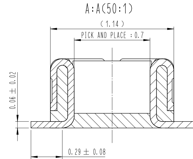
ENGAGEMENT FIGURE (50:1)
