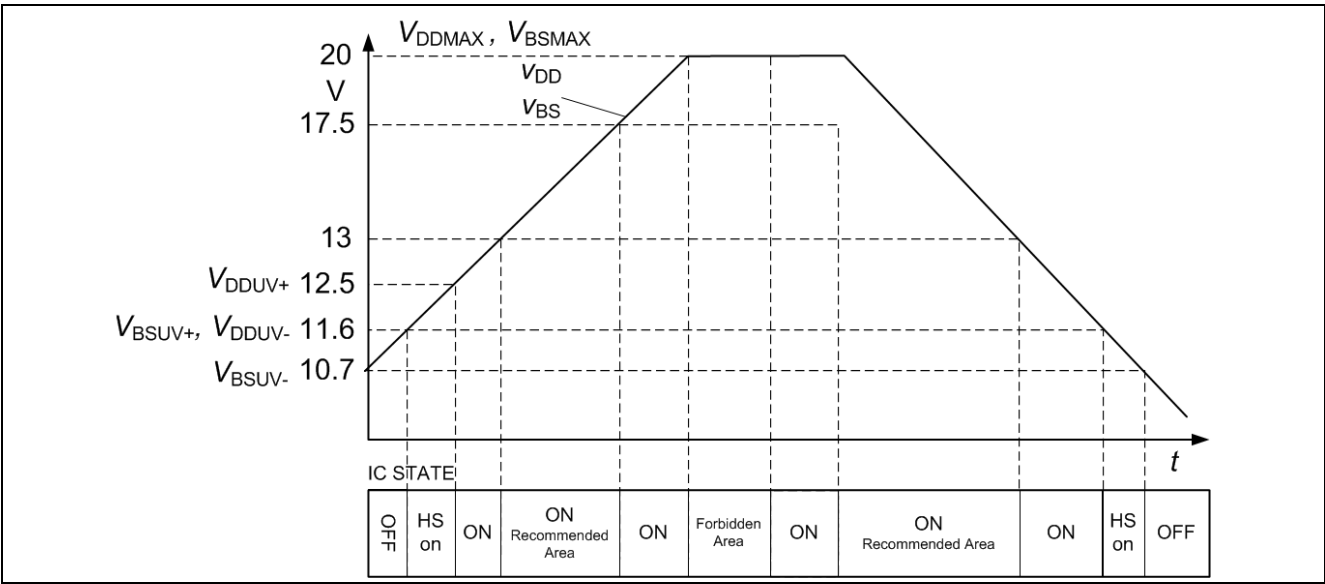
Figure 20 Operating areas (IGBT UVLO levels)
