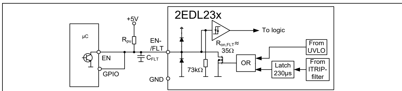
Figure 6 EN-/FLT pin structures and interface to microcontroller ( \mu C)
