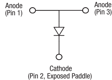
Figure 1. CLA4609-086LF Block Diagram
