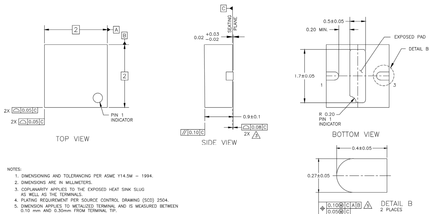
Figure 9. CLA4609-086LF Package Dimensions
