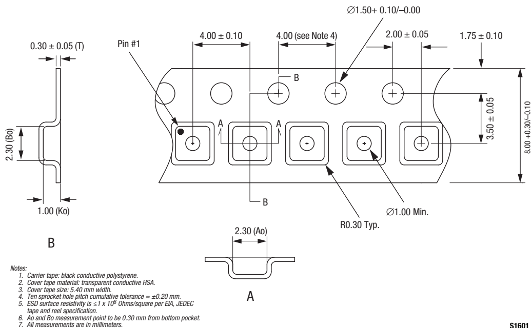
Figure 10. CLA4609-086LF Tape and Reel Dimensions
