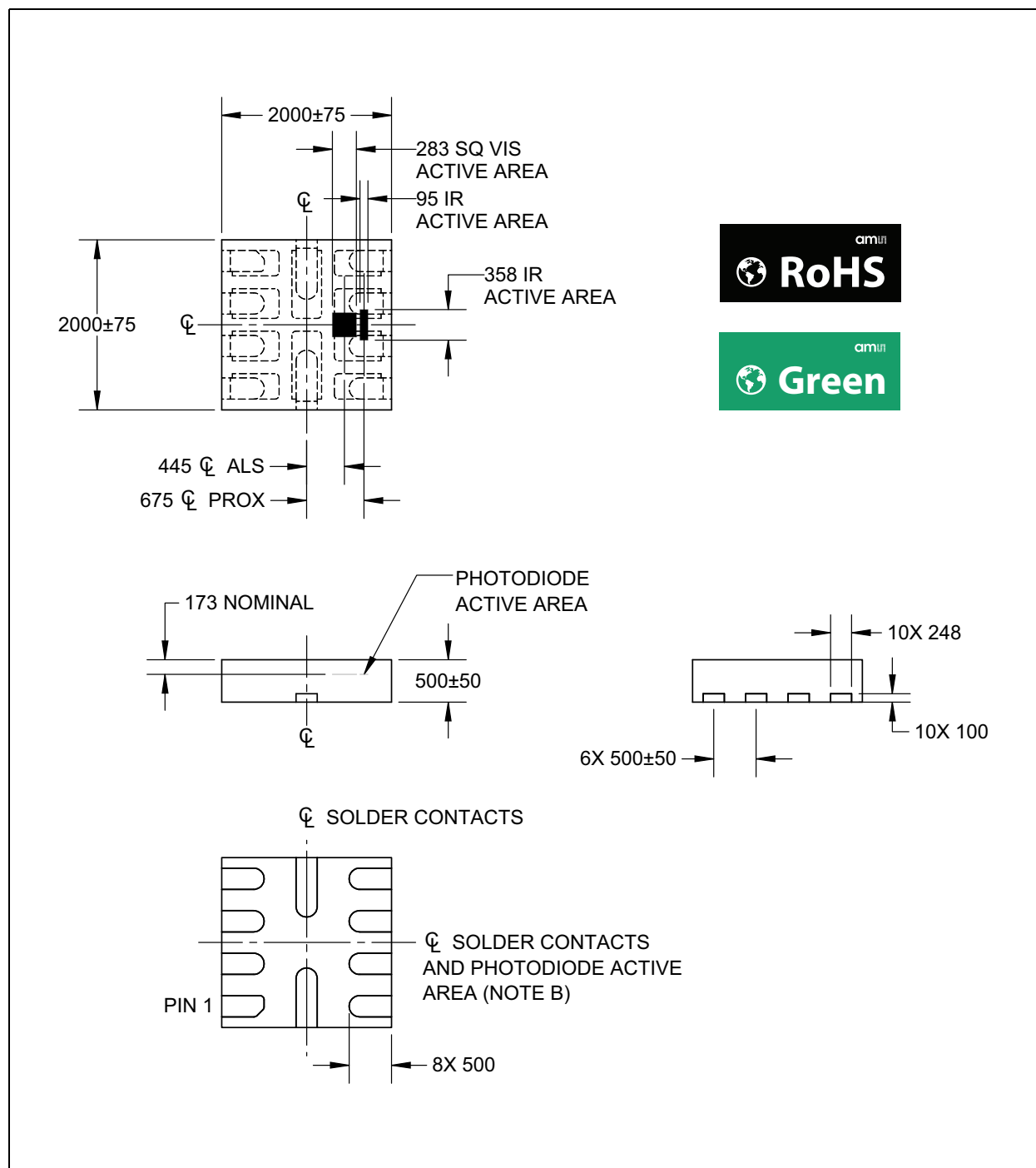
Figure 38: Package Drawing
