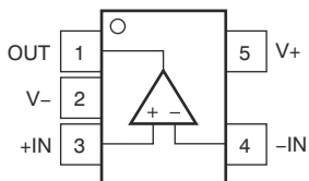
Figure 5-2. OPA140: DBV Package, 5-Pin SOT-23 (Top View)
