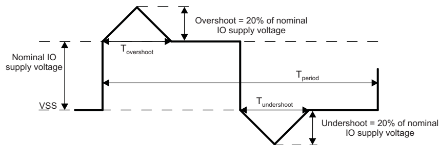
Figure 5-1. T_{\text{overshoot}} + T_{\text{undershoot}} < 20\% of T_{\text{period}}
