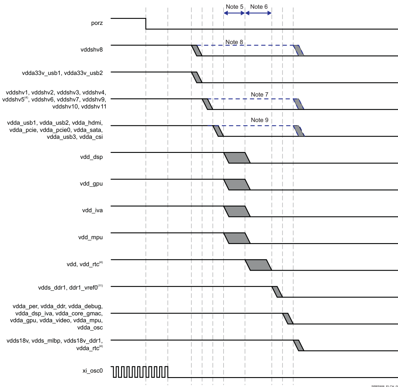
Figure 5-3. Power-Down Sequencing (10)(12)
