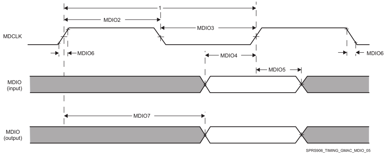
Figure 7-55. GMAC MDIO diagrams
