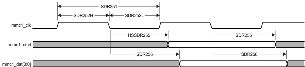
Figure 7-67. MMC/SD/SDIO in - High Speed SDR25 - Transmitter Mode
