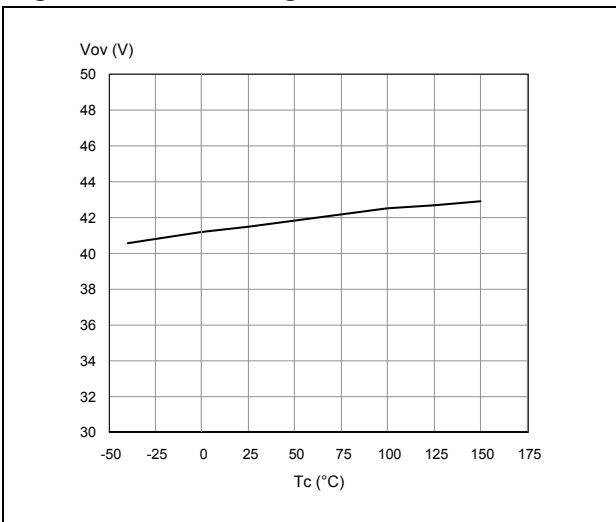
Figure 11. Overvoltage shutdown
