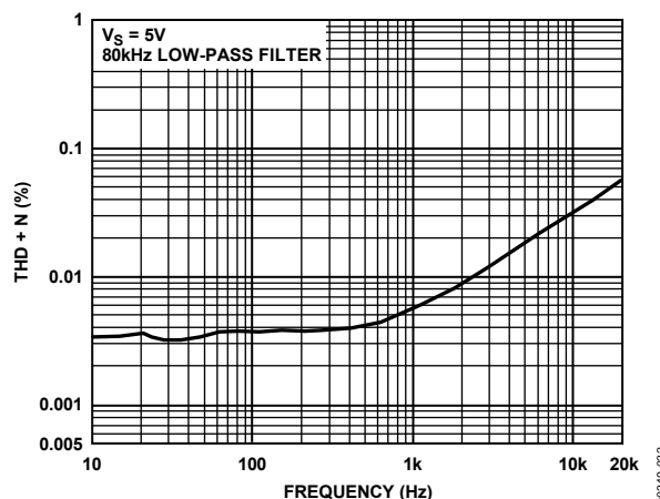
Figure 32. Headphone Driver THD + N vs. Frequency into a 32\ \Omega Load
