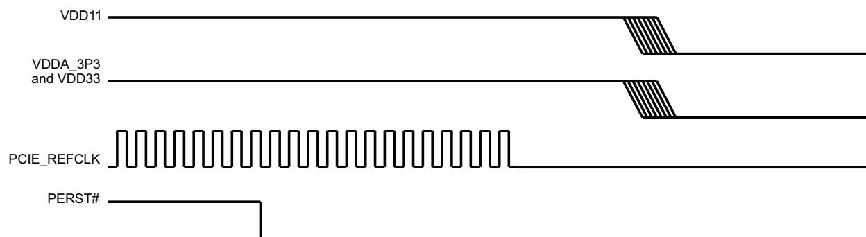
Figure 24. Power-Down Sequence
