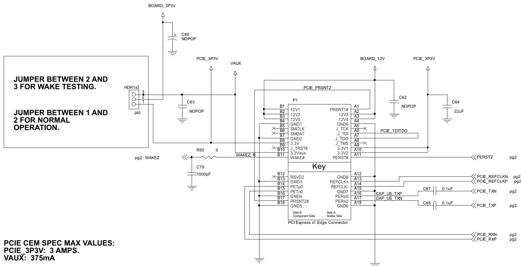
Figure 12. Reference Design 3
