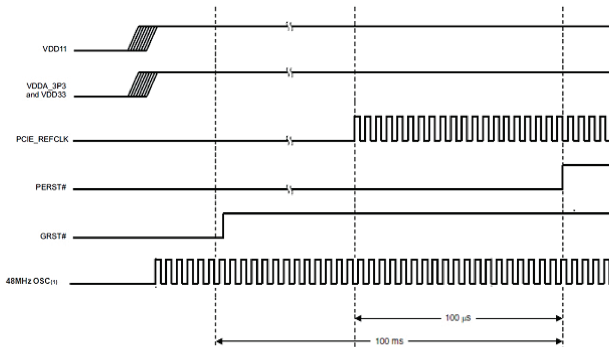
Figure 23. Power-Up Sequence
