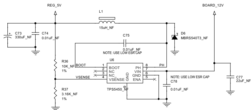
Figure 14. Reference Design 5
