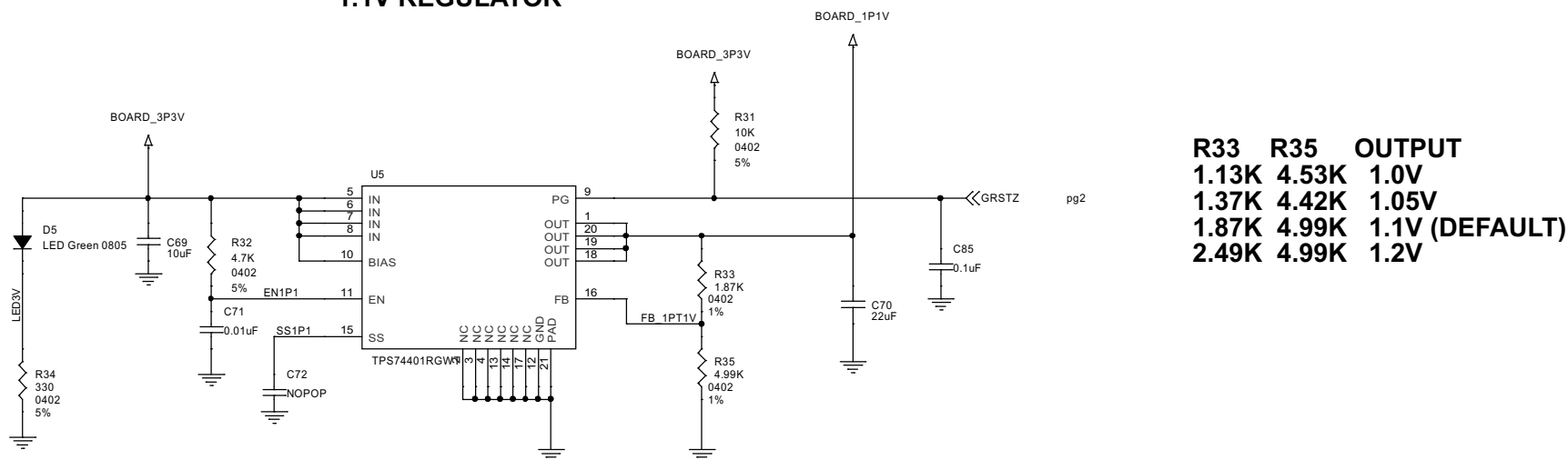
Figure 13. Reference Design 4
