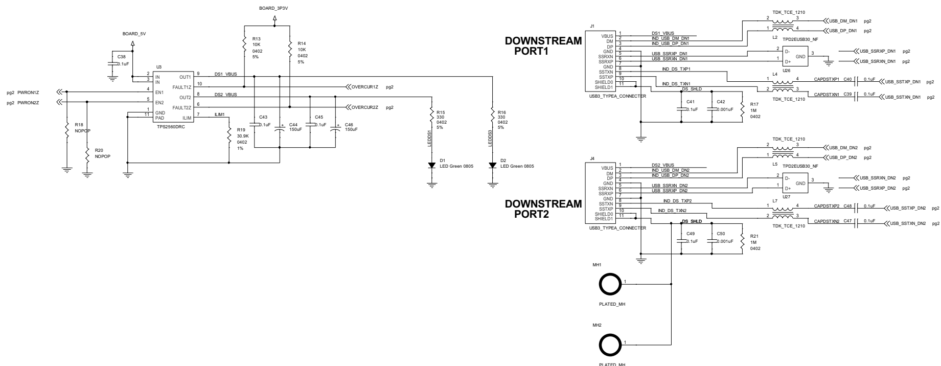
Figure 11. Reference Design 2
