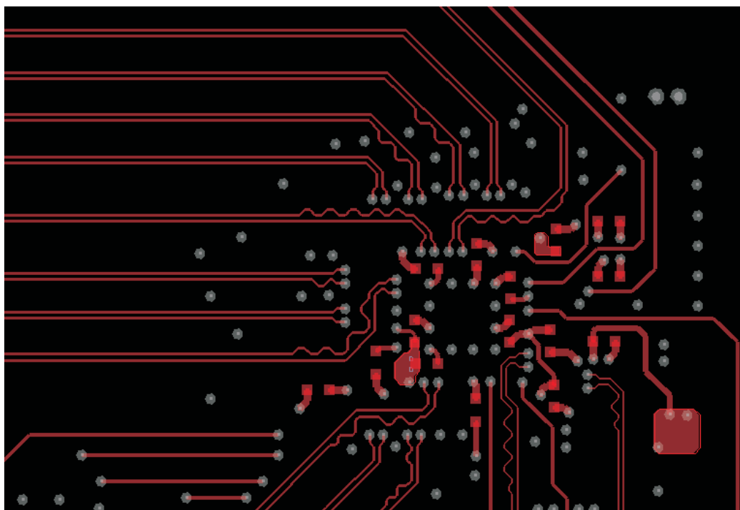
Figure 26. Length Matching
