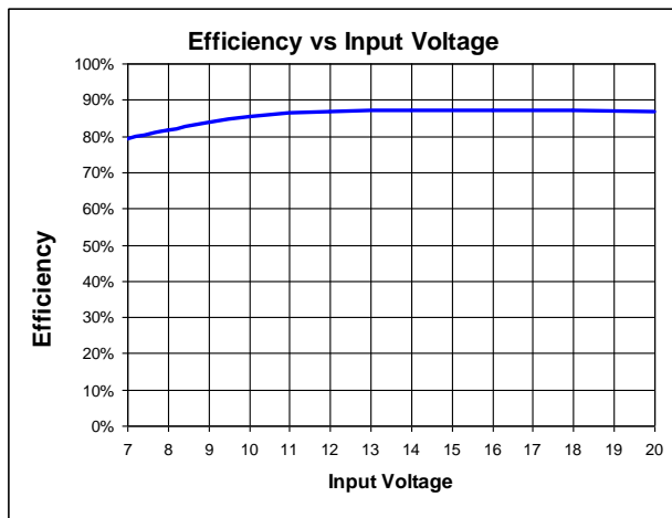
Figure 47 Efficiency
