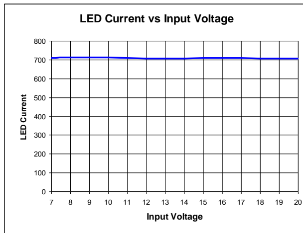
Figure 48 Line Regulation
