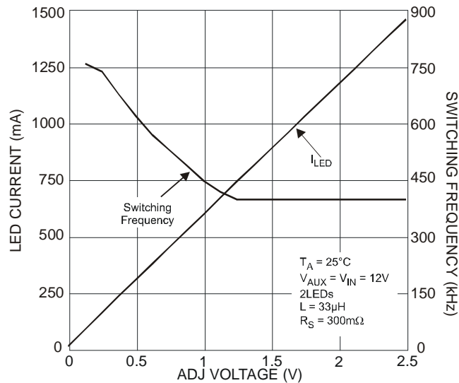
Figure 5 Buck LED Current, Switching Frequency vs. V_{ADJ}
