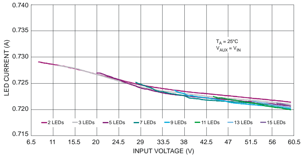
Figure 12 I_{\text{LED}} vs. Input & Number of LED
