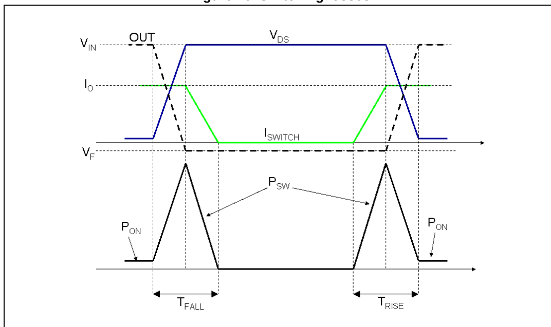
Figure 16. Switching losses
