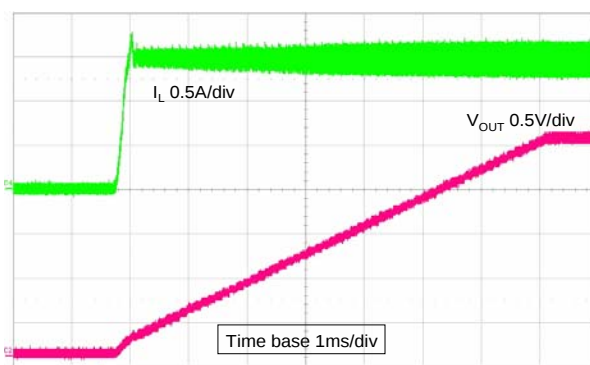
Figure 31. Soft-start
