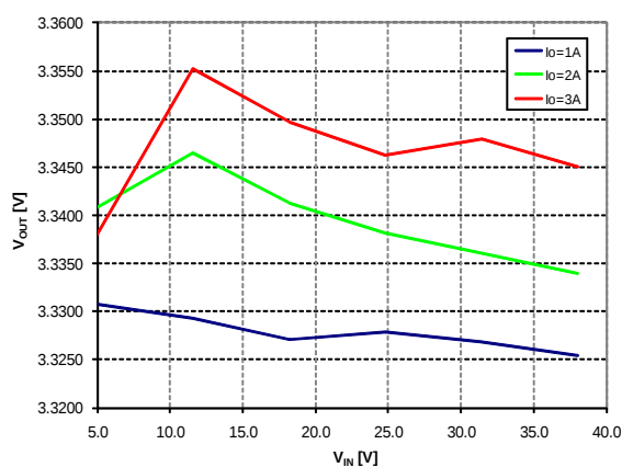
Figure 29. Line regulation
