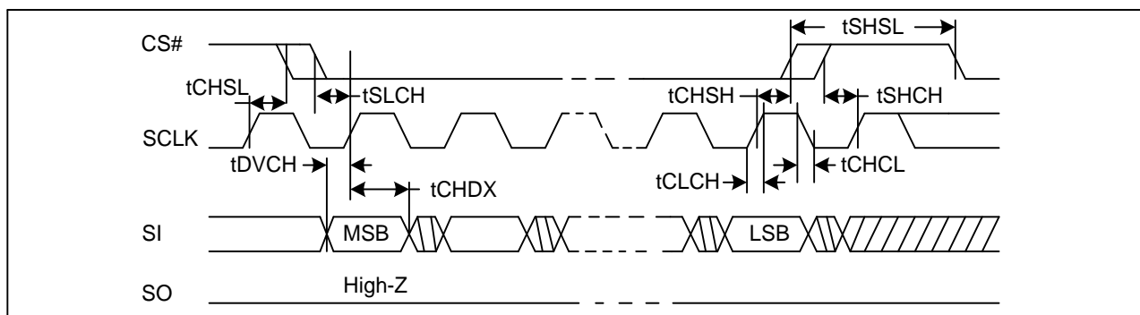
Figure 39. Input Timing
