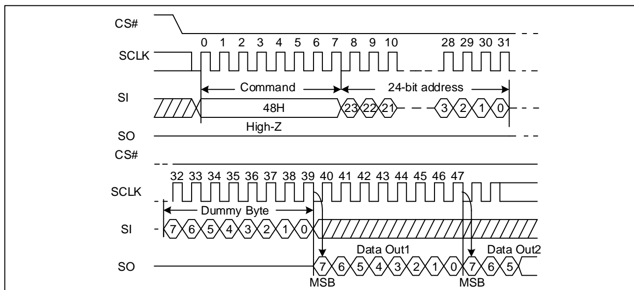
Figure 28. Read Security Registers command Sequence Diagram
