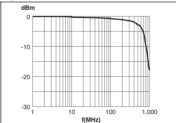
Figure 18. DALC208SC6 attenuation
