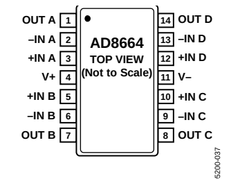
Figure 6. AD8664, 14-Lead TSSOP (RU-14)
