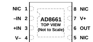
Figure 2. AD8661, 8-Lead LFCSP (CP-8-13)
