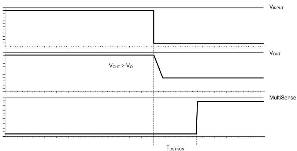
Figure 8. T_{\text{DSTKON}}
