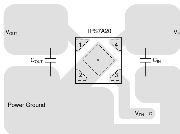
Figure 10-2. DQN Package (X2SON) Typical Layout
