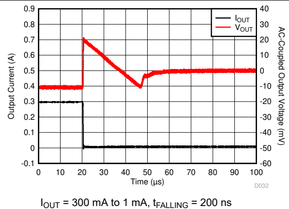
Figure 6-54. Load Transient
