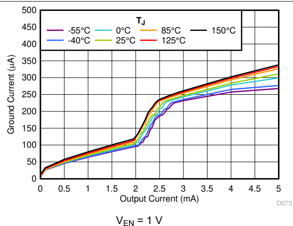
Figure 6-40. I_{GND} vs I_{OUT}
