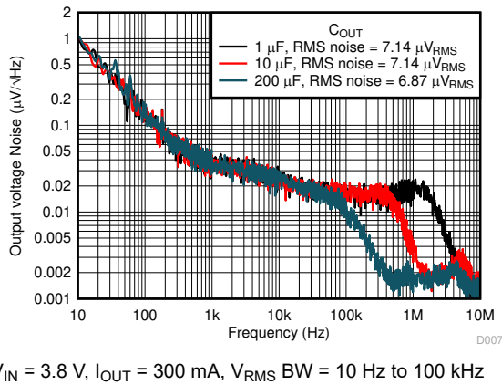
Figure 6-69. Noise vs Frequency and C_{OUT}
