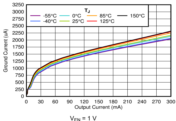
Figure 6-38. I_{GND} vs I_{OUT}
