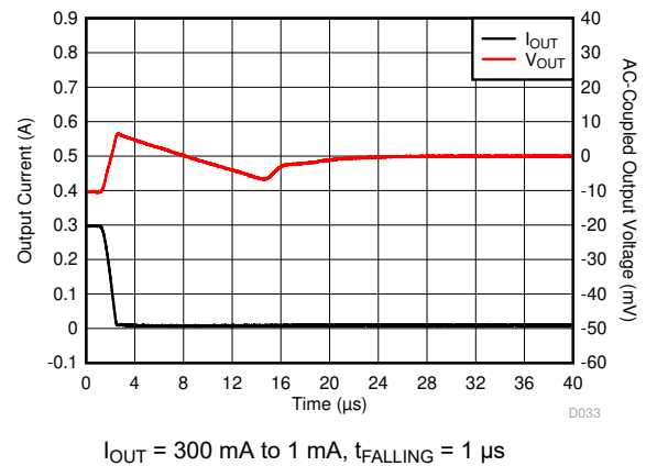
Figure 6-52. Load Transient
