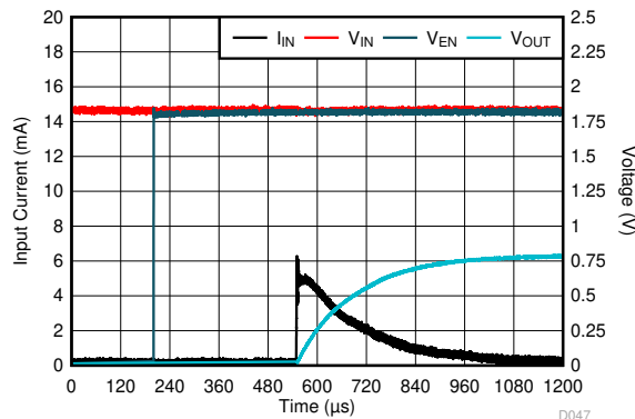
Figure 6-81. Startup
