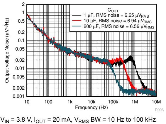
Figure 6-68. Noise vs Frequency and C_{OUT}
