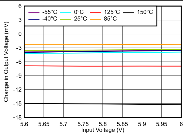
Figure 6-2. Line Regulation vs V_{IN}
