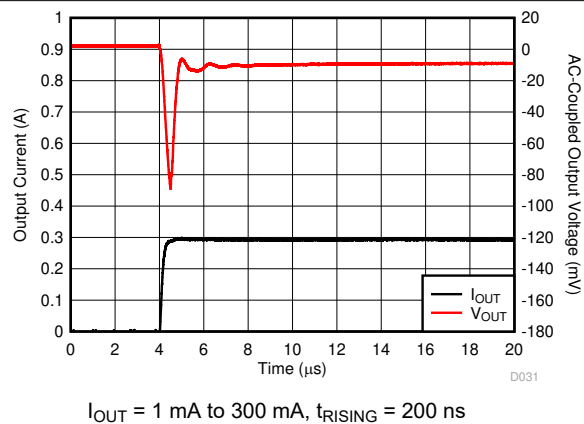
Figure 6-53. Load Transient
