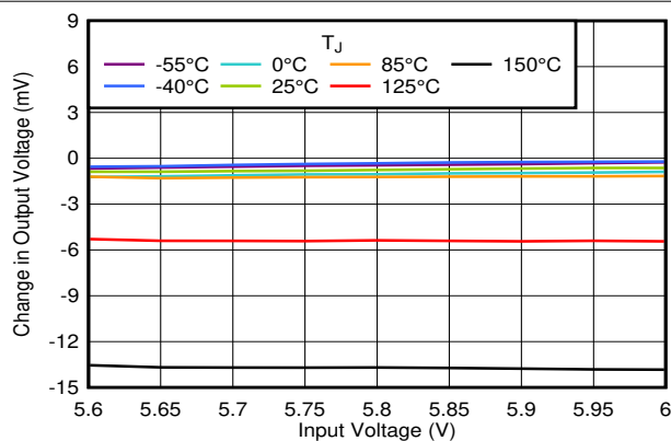
Figure 6-2. Line Regulation vs V_{IN}
