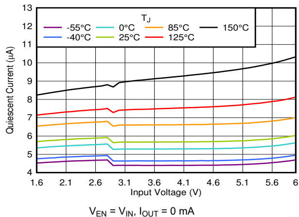
Figure 6-35. I_{GND} vs V_{IN}
