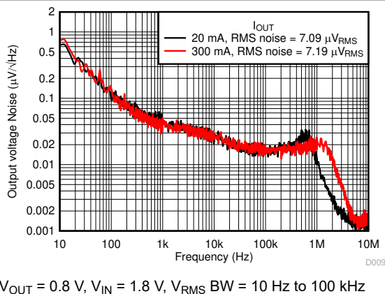
Figure 6-71. Noise vs Frequency and I_{OUT}
