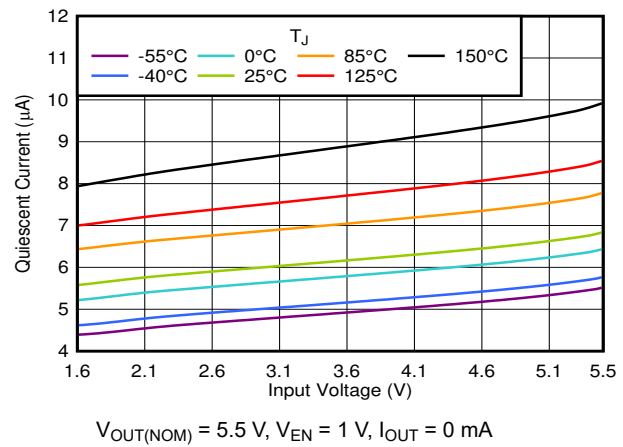
Figure 6-36. I_{GND} vs V_{IN} in the Dropout Region
