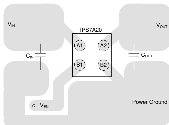
Figure 10-3. YCK Package (DSBGA) Typical Layout
