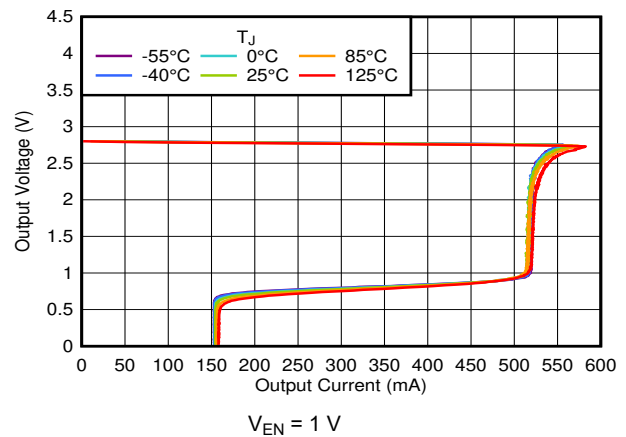
Figure 6-44. Current Limit
