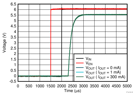
Figure 6-79. Startup
