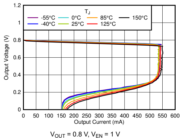
Figure 6-45. Current Limit
