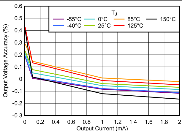
Figure 6-14. Output Voltage Accuracy vs I_{OUT}
