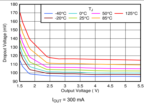
Figure 6-33. Dropout Voltage vs V_{OUT}
