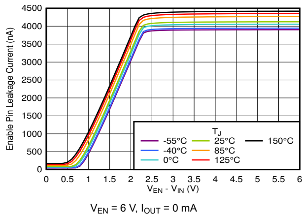
Figure 6-43. Enable Pin Leakage Current vs V_{EN} - V_{IN}
