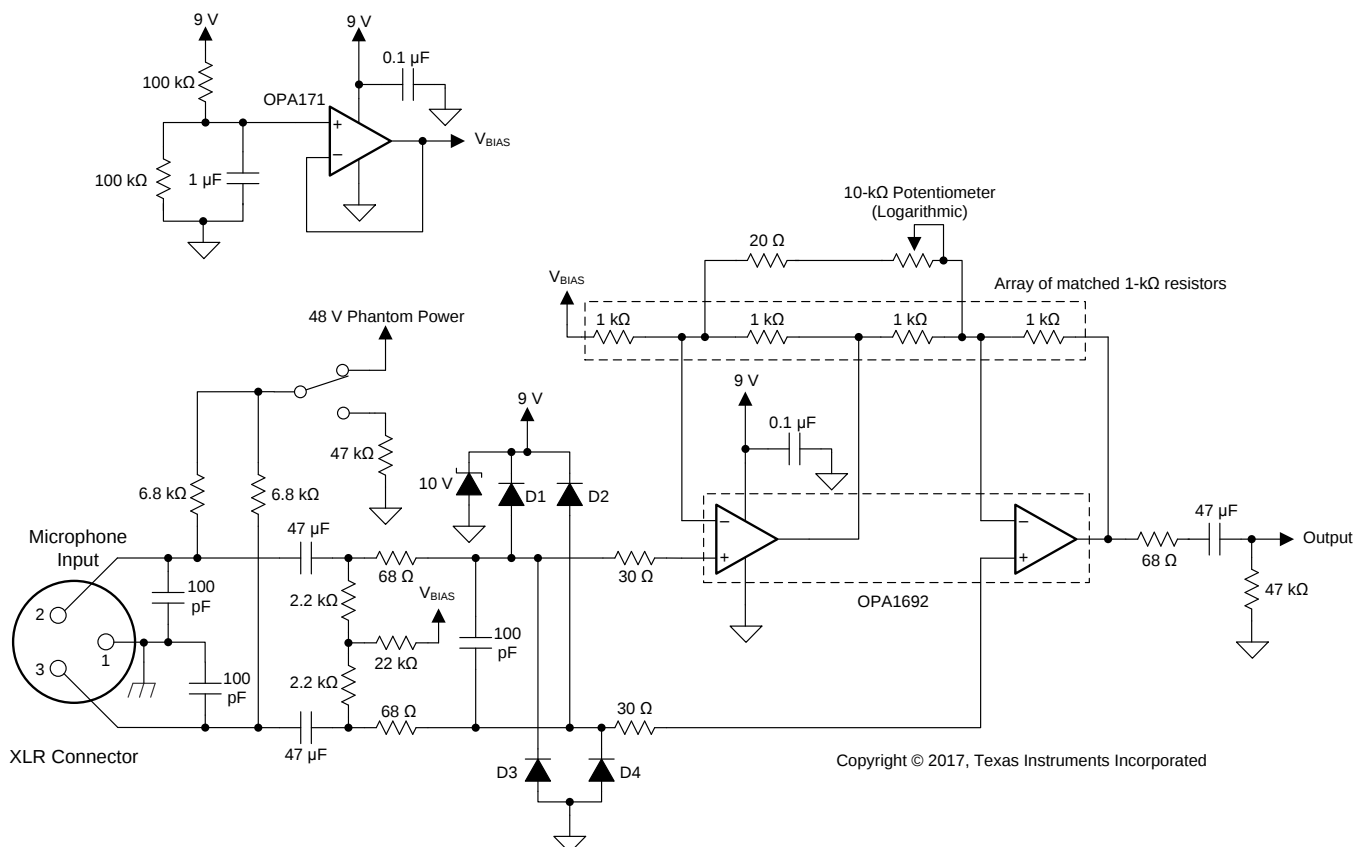
Figure 63. Preamplifier for Professional Microphones Powered from a 9-V Battery
