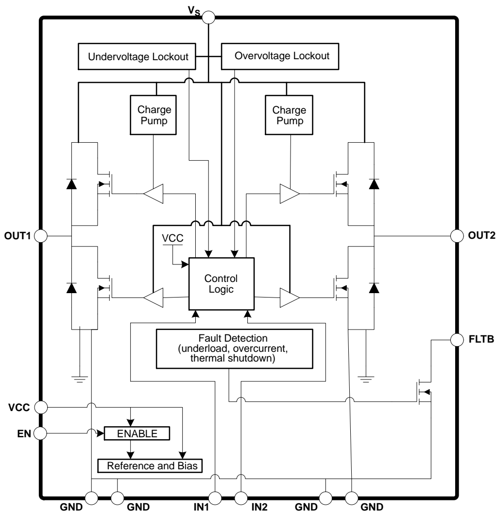
Figure 2. Block Diagram
