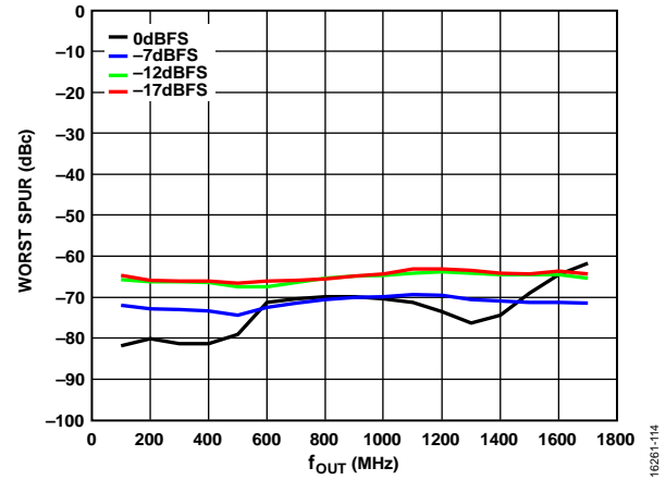
Figure 14. Worst Spur (dBc) vs. f_{OUT} over Digital Scale (Mode 17), 3.4 GHz DAC Sample Rate, Channel Interpolation 1 \times , Main Interpolation 1 \times , 11-Bit Resolution
