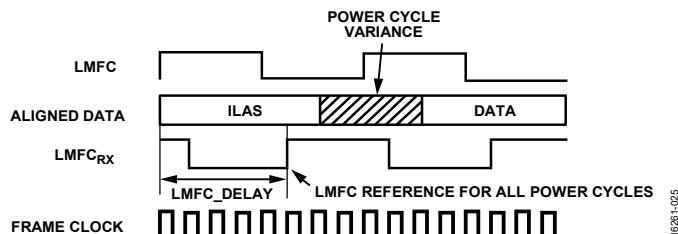
Figure 63. LMFC_DELAY_x to Compensate for Link Delay > LMFC
