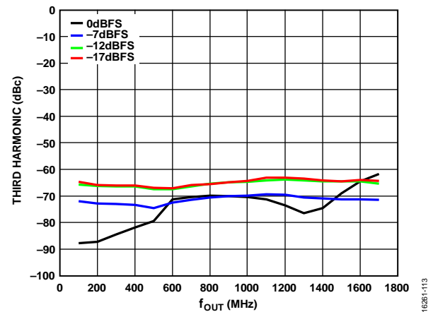
Figure 13. Third Harmonic (dBc) vs. f_{OUT} over Digital Scale (Mode 17), 3.4 GHz DAC Sample Rate, Channel Interpolation 1 \times , Main Interpolation 1 \times , 11-Bit Resolution
