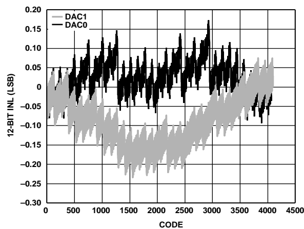
Figure 42. INL, I_{OUTFS} = 20 mA, 12-Bit Resolution
