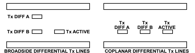
Figure 85. Broadside vs. Coplanar Differential Stripline Routing Techniques
