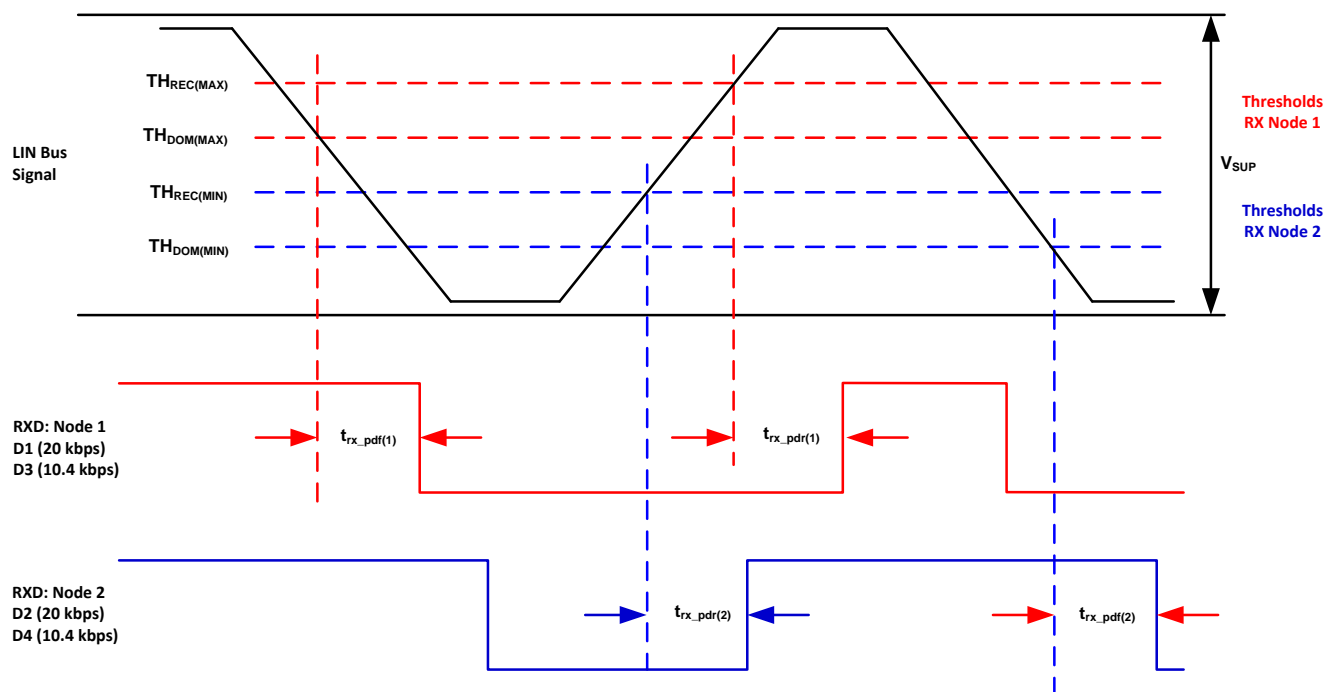
Figure 21. Propagation Delay
