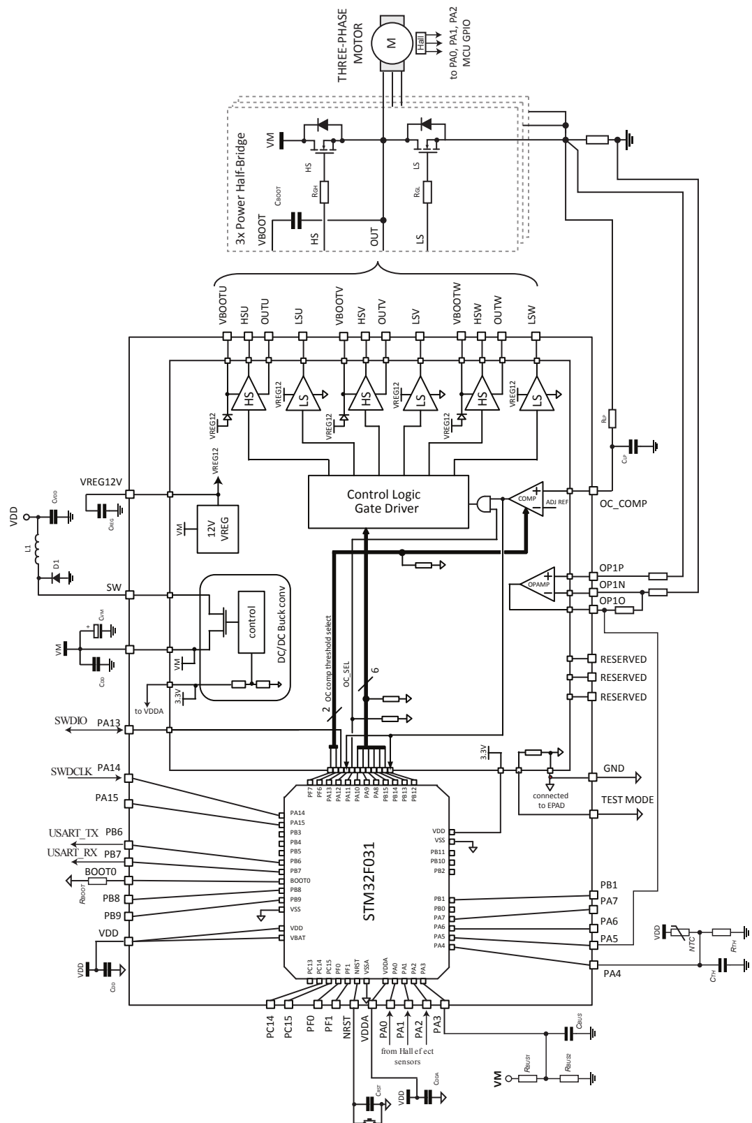
Figure 19. Application example
