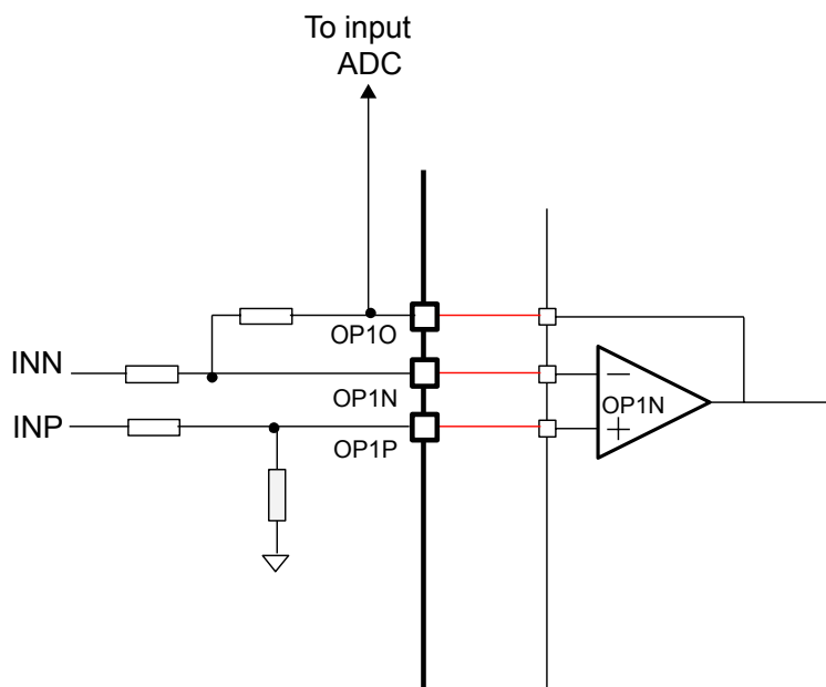
Figure 15. Operational amplifier
