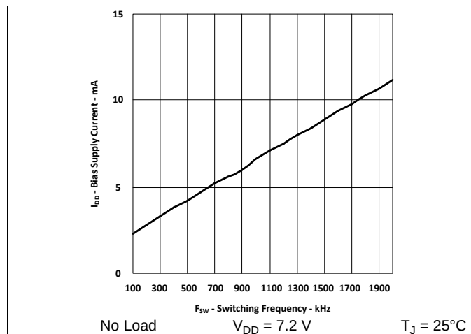
Figure 14. Bias Supply Current vs Switching Frequency
