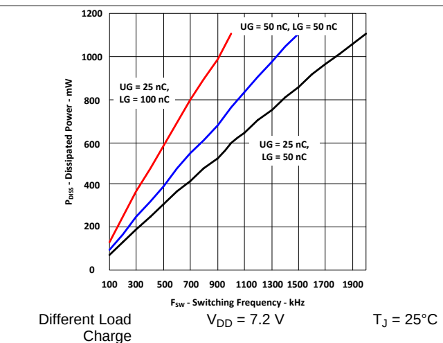
Figure 15. Driver Dissipated Power vs Switching Frequency
