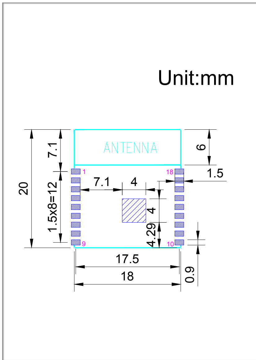
Figure 7-1. Recommended PCB Land Pattern of ESP-WROOM-02
