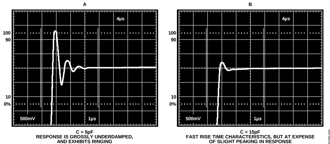
Figure 49. Effect of Altering Compensation from Circuit in Figure 47—PM7545 CMOS DAC with 1/2 OP249, Unipolar Operation; Critically Damped Response Is Obtained with C ≈ 33 pF
