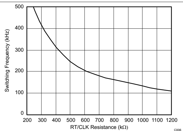
Figure 32. Low-Range RT
