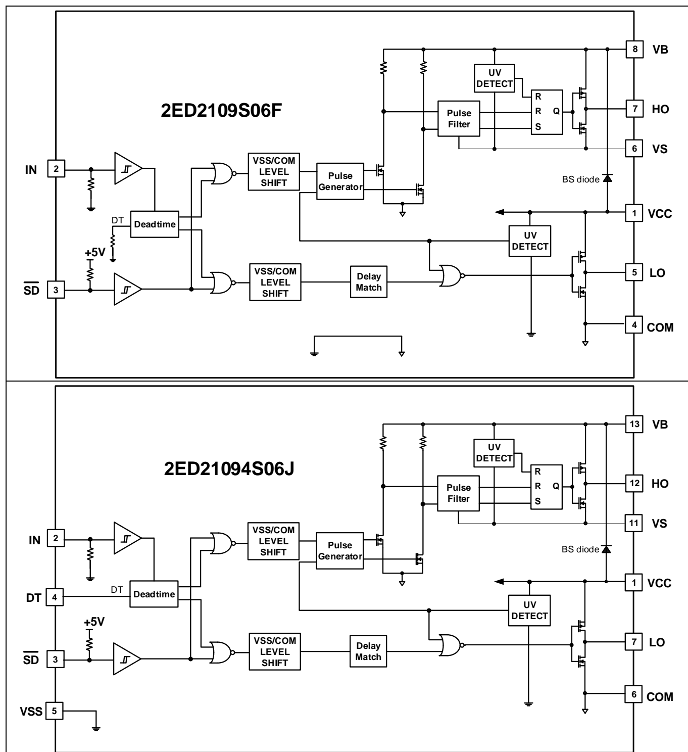
Figure 2 Block diagrams
