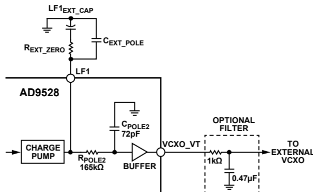
Figure 28. PLL1 Loop Filter
