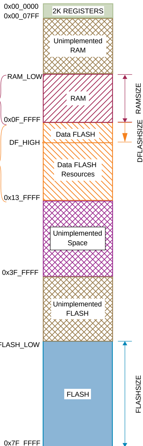
Figure 3-19. S12X CPU & BDM Global Address Mapping
