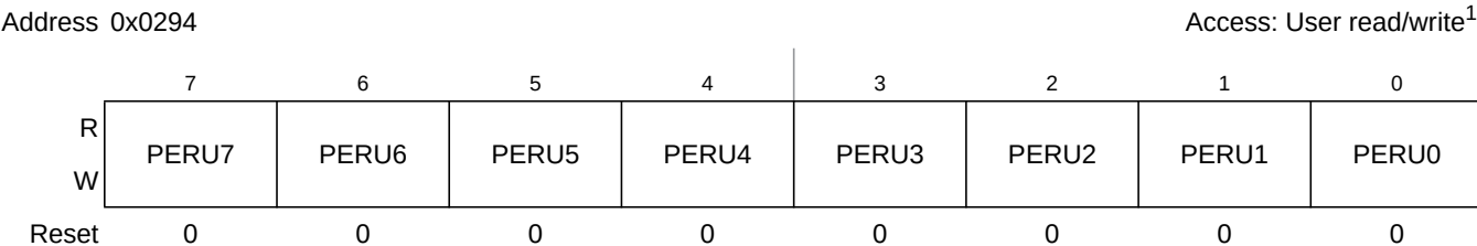
Figure 2-82. Port U Pull Device Enable Register (PERU)
