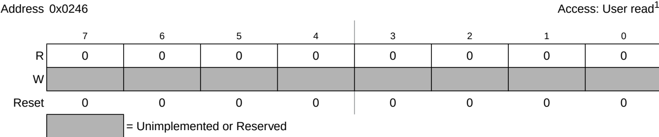
Figure 2-18. PIM Reserved Register
