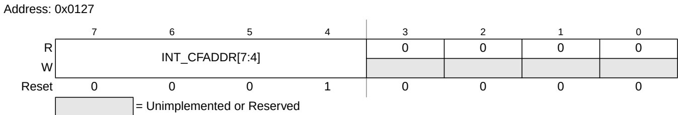
Figure 4-5. Interrupt Configuration Address Register (INT_CFADDR)
