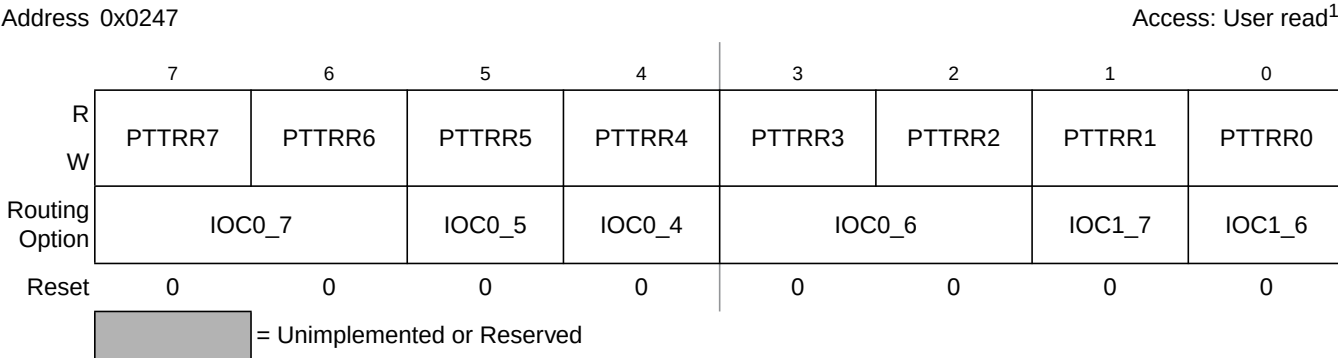
Figure 2-19. Port T Routing Register (PTTTR)
