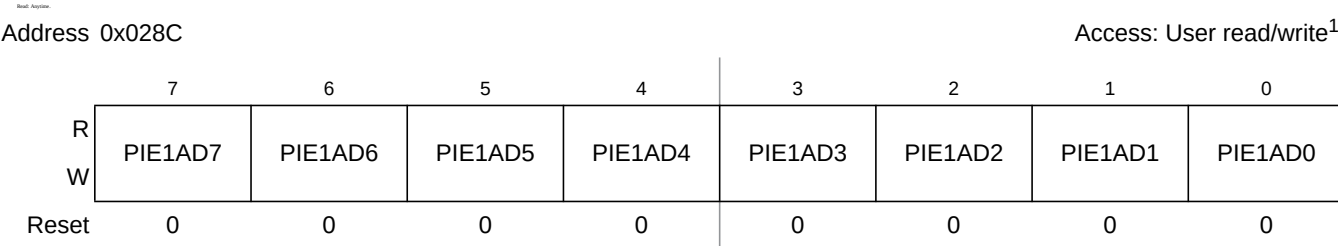
Figure 2-74. Port AD Interrupt Enable Register (PIE1AD)
