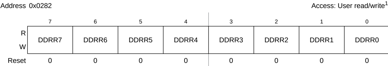
Figure 2-64. Port R Data Direction Register (DDRR)
