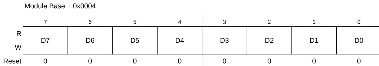
Figure 12-8. IIC Bus Data I/O Register (IBDR)
