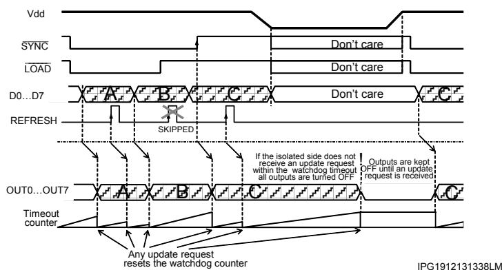
Figure 7. Watchdog behavior
