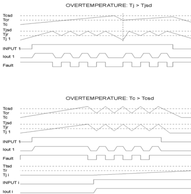
Figure 18. Thermal protection
