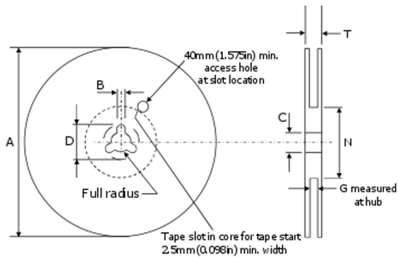
Figure 27. Reel specifications
