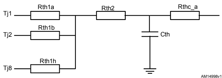
Figure 22. Simplified thermal model
