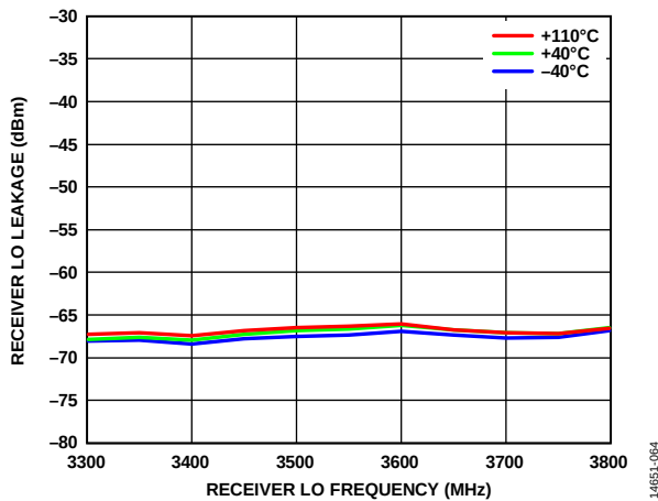
Figure 123. Receiver Local Oscillator (LO) Leakage vs. Receiver LO Frequency, 0 dB Receiver Attenuation, 100 MHz RF Bandwidth, 153.6 MSPS Sample Rate
