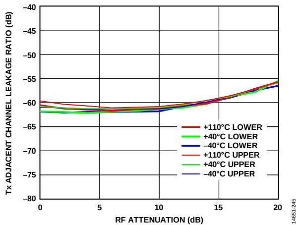
Figure 206. Tx Adjacent Channel Leakage Ratio vs. RF Attenuation, 5600 MHz LO, 75 MHz RF Bandwidth, Four-Carrier W-CDMA Desired Signal, Transmitter QEC and LO Leakage Tracking Active
