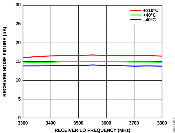
Figure 125. Receiver Noise Figure vs. Receiver LO Frequency, 0 dB Receiver Attenuation, 100 MHz RF Bandwidth, 153.6 MSPS Sample Rate, 50 MHz Integration Bandwidth (Includes 1 dB Matching Circuit Loss)
