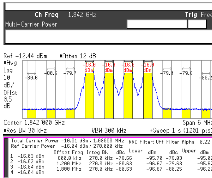
Figure 70. Four-Carrier MC-GSM, IF = 30 MHz ACPR, LO Frequency = 1812 MHz
