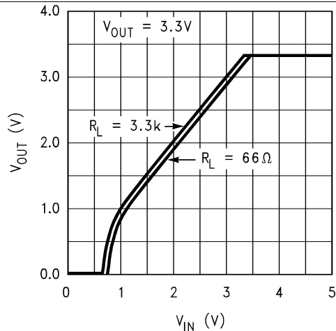
Figure 5. Dropout Characteristics
