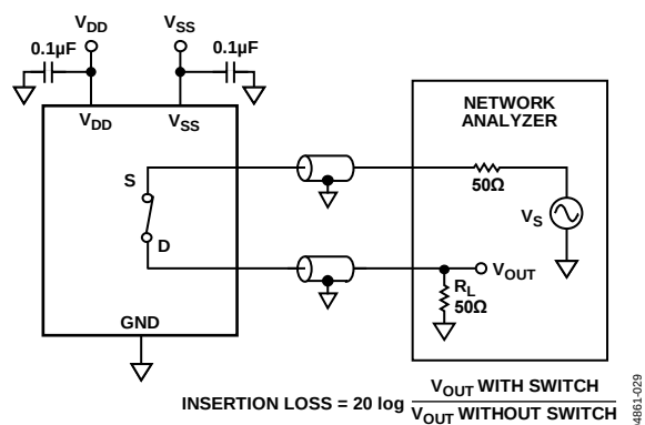
Figure 35. Insertion Loss
