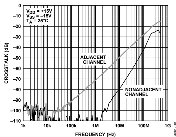
Figure 21. ADG1409 Crosstalk vs. Frequency
