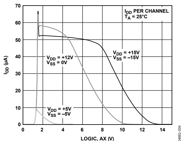
Figure 16. Positive Supply Current vs. Logic Level
