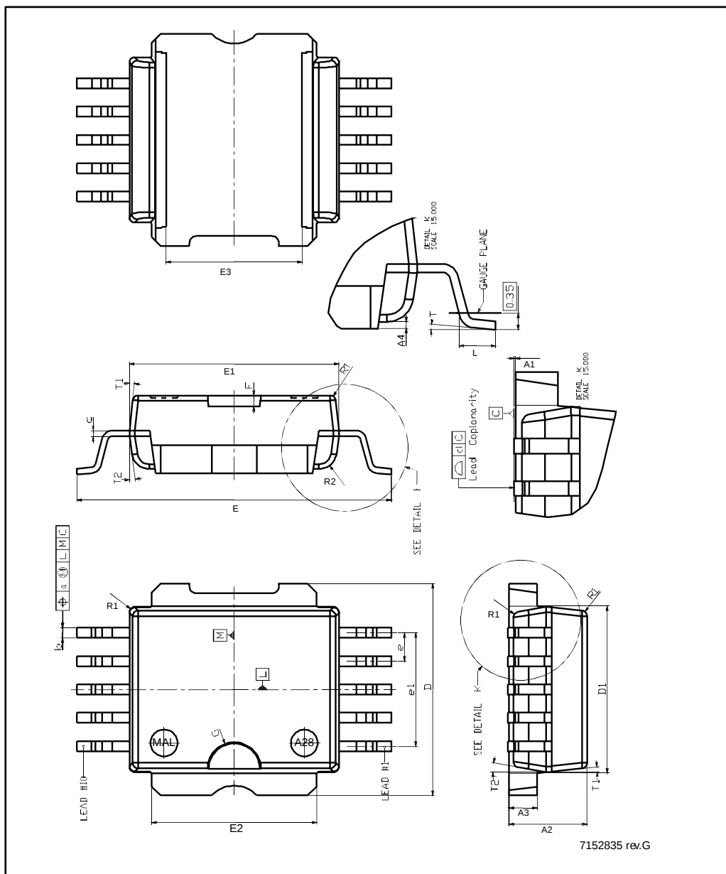
Figure 10: PowerSO-10 package outline
