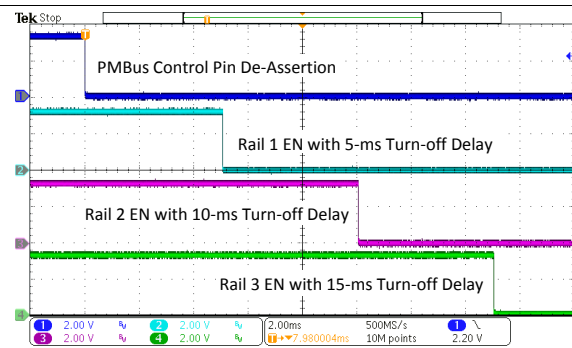
Figure 34. Example Power-Off Sequence
