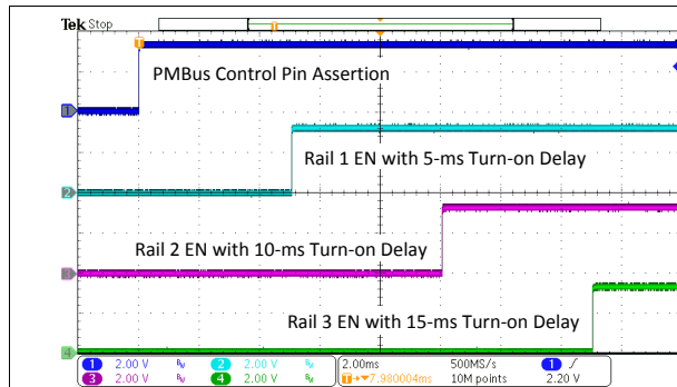
Figure 33. Example Power-On Sequence
