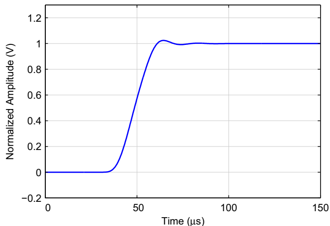
Figure 9-56. Step Response
