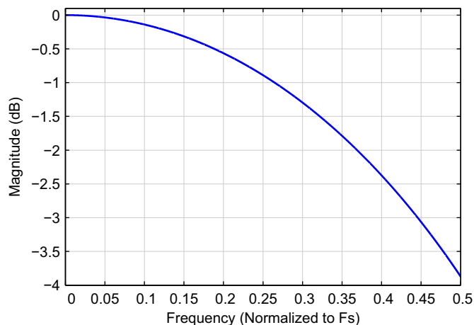
Figure 9-57. Passband Ripple
