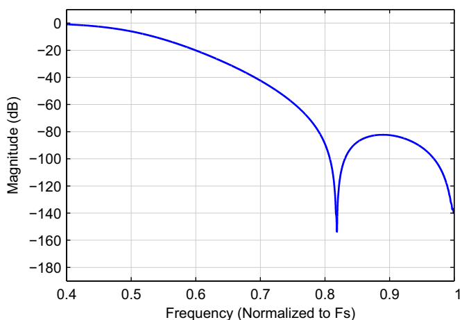
Figure 9-26. Stopband Attenuation
