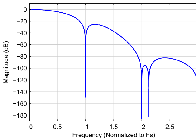
Figure 9-58. Stopband Attenuation
