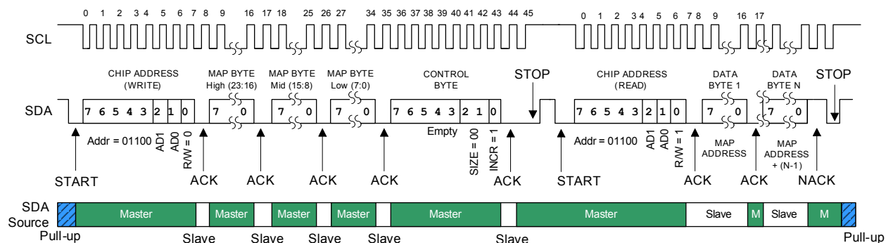
Figure 4-34. Control Port Timing, I²C Reads with Preamble and Autoincrement (8-Bit Data Access)
