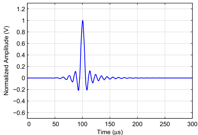
Figure 9-45. Impulse Response—Linear Phase
