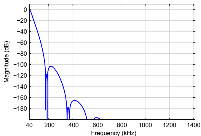
Figure 9-67. Stopband Attenuation
