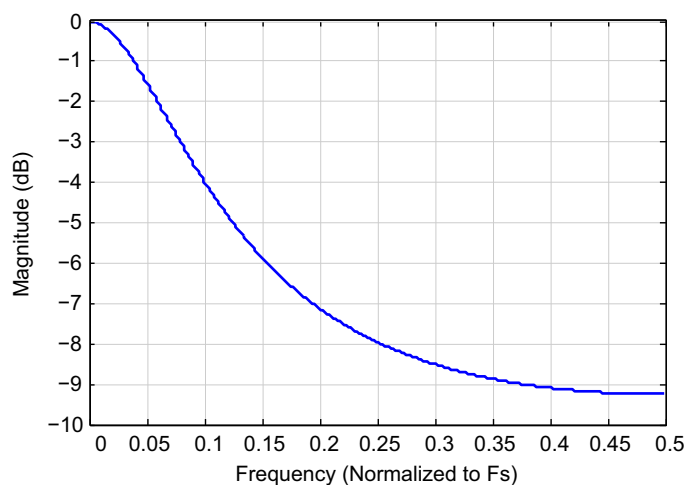
Figure 9-71. Deemphasis
