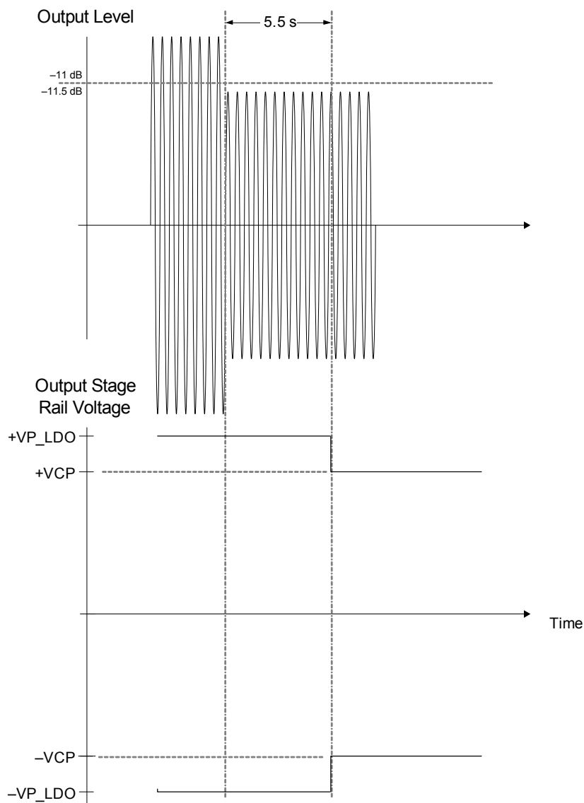
Figure 4-5. VCP_FILT Hysteresis
