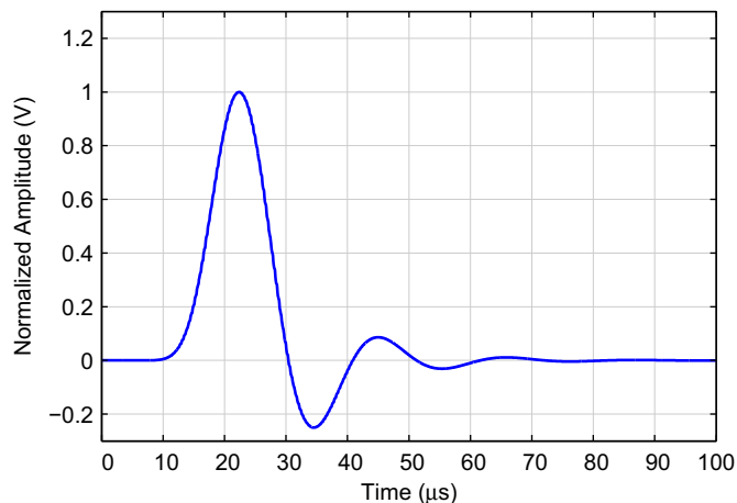
Figure 9-68. Impulse Response
