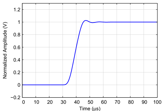
Figure 9-60. Step Response
