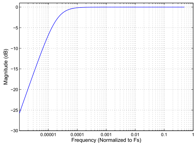
Figure 9-70. Highpass Filter for PCM and DSD Paths
