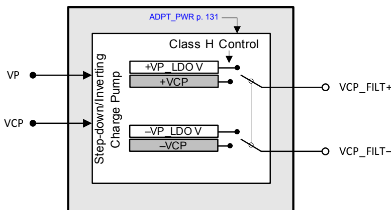
Figure 4-2. Class H Operation
