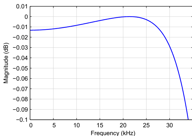
Figure 9-66. Passband Ripple
